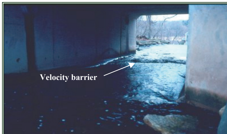
Figure 4. Example of excessive water velocities resulting in a barrier to fish passage.
